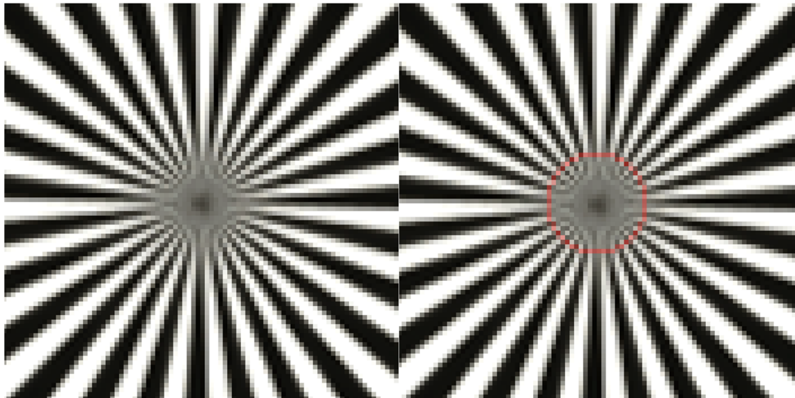
Fig. 5: Blur radius for the panchromatic sensor on a white siemens star, blur radius of 11 pixel
