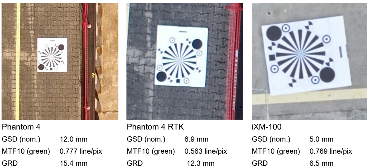
Fig. 1: Siemens star image and analysis from Phantom 4 (left), Phantom 4 RTK (middle) and Phase One iXM100-RS (right). Each image sample is sized 300 x 300 pix.
