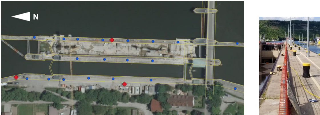
Fig. 3: Test area of ship lock Hessigheim/Neckar with distribution of signalized points. The image on the right shows one of the signalized points. All points are fixed to the ground except three, which are mounted on top of approximately 140 cm high concrete pillars (red squares).
