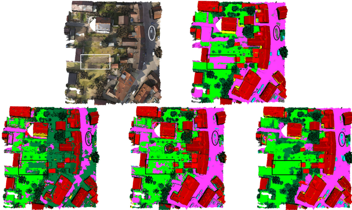
Fig. 4: Ground truth and predictions of several classifiers on tile C. The feature vector consists of XYZ , normal vector and median HSV (face) . Top row : Tile C colored with median RGB per face ( left ) and ground truth ( right ). The oval shows cars labeled as clutter (label noise) that are consistently predicted as vehicle for PointNet/PointNet++. Bottom row (from left to right) : RF (OA = 69.54 % and mIoU = 22.46 %), PointNet (OA = 70.89 %; mIoU = 29.44 %), PointNet++ (OA = 80.62 %; mIoU = 43.54 %). The circle shows a false prediction ( roof, chimney/antenna ) for a tree due to feature encoding at global scale (PointNet). The rectangle shows that all classifiers have issues separating green space from impervious surface . Best viewed digitally.
